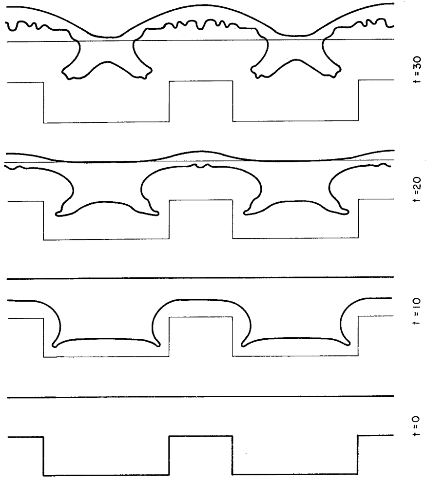
Fig. 9 Successive configurations of gas slab with wide internal flanges; density ratio R = 1 .
